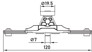
W3719侧压上轮 编号:R00668
