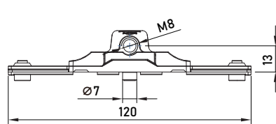
W3719侧压中间锁 编号:R00669
