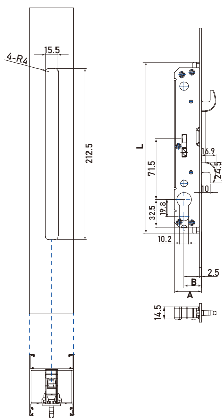
Milling Dimension
