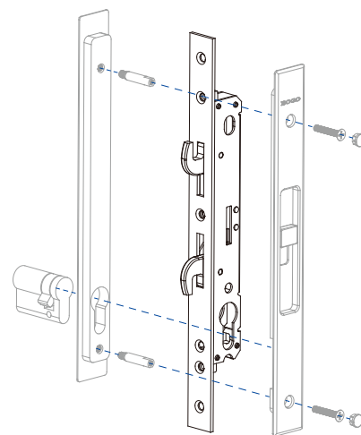
Typical Installation
